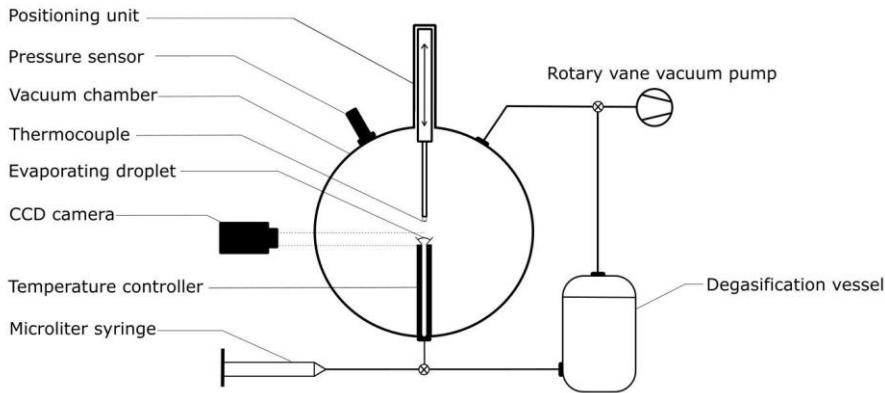
Figure 1. (Left) Schematic overview of the experimental set-up and (right) front view of the experimental setup with the glass window through which the camera can measure the height of the droplet.
